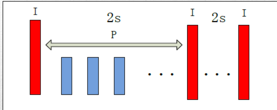
Figure 3 Fixed GOP
