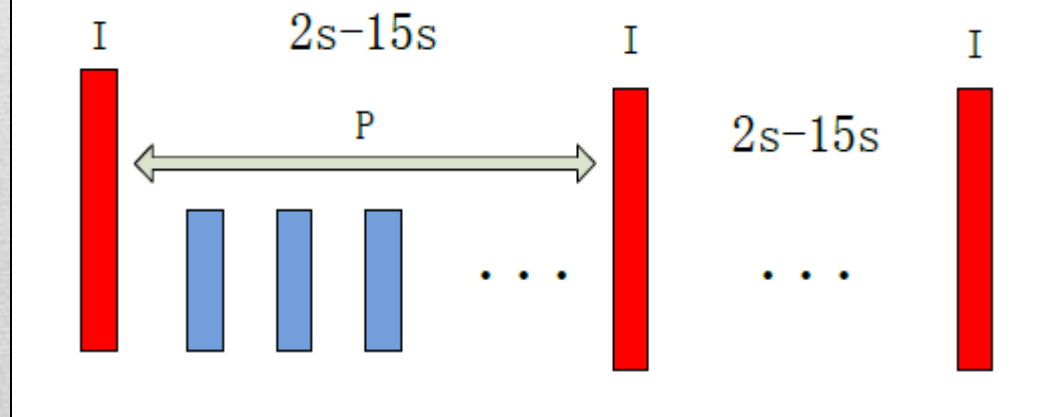
Figure 3 Fixed GOP
